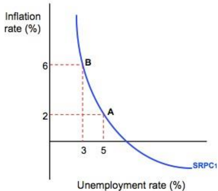
Short-run Phillips curve:
